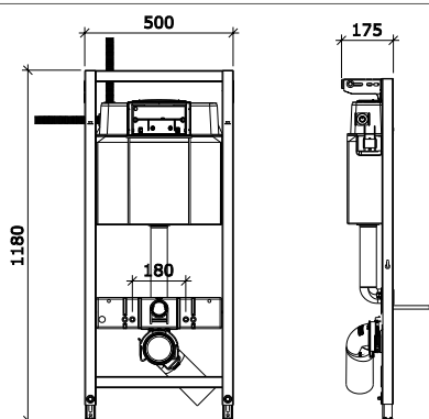
5970-10 Bano standard fixtur/cistern
